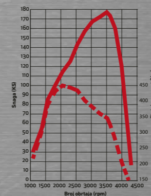
— Snaga ···· Obrtni momenat
